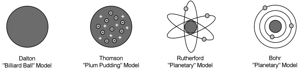
Fig. 7: The Dalton (1805), Thomson (1904), Rutherford (1911), and Bohr (1913) models of the atom with their corresponding analogies.
