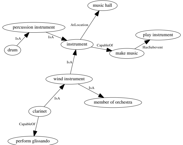
Fig. 12: Experiment 1: Evolved individual, 10 concepts, 9 relations (target domain). The evolved individual is encountered after 42 generations, with fitness value 2.7. Concepts and relations of the individual not involved in the analogy are not shown here for clarity.
