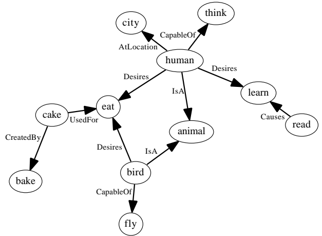
Fig. 1: A semantic network with 11 concepts and 11 relations.
