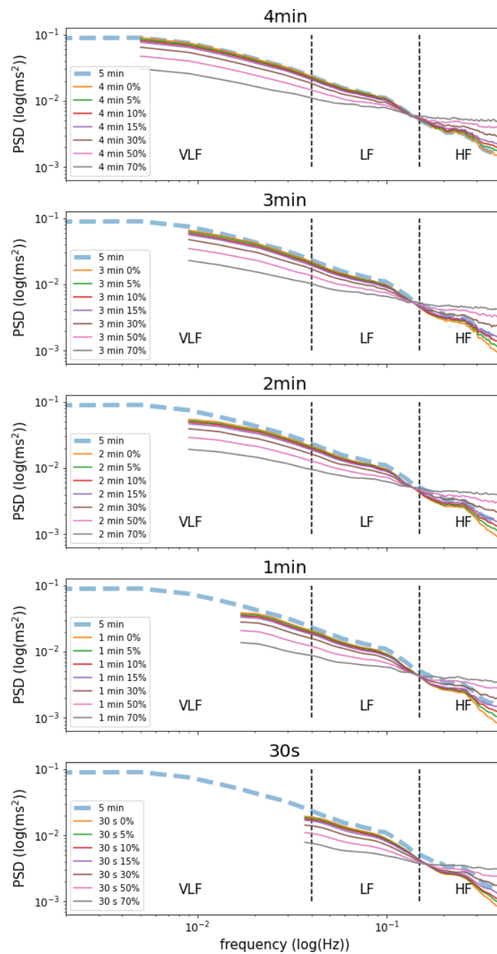
Figure 1. Power Spectrum Density plot for timeseries with different time series length and missing values percentage. The blue dotted line in each plot reflects the power spectrum of the 5 min time window.
