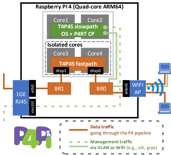
Figure 1: Overview of the P4Pi architecture
