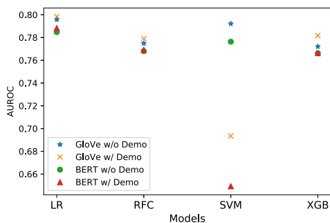
Fig. 4. Average AUROC for the four baseline models. We compared four sets of input, GloVe embeddings without demographics (‘GloVe w/o Demo’), GloVe embeddings with demographics (‘GloVe w/ Demo’), BERT embeddings without demographics (‘BERT w/o Demo’) and BERT embeddings with demographics (‘BERT w/ Demo’).
