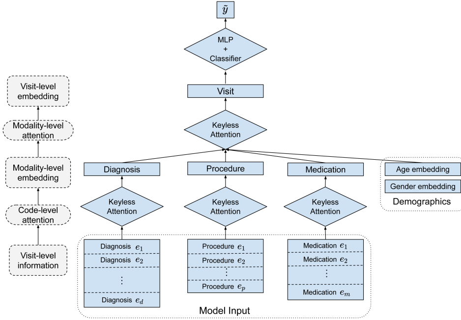
Fig. 1. Illustration for the Dual Keysless Attention (DuKa) Model. The e in the Model Input box represents the pre-trained embeddings and its subscriptions d, p and m represent the number of diagnosis, procedure and medication codes in a visit, respectively. Notably, the age and gender embeddings are randomly initialised which follows the practices implemented in [21].
