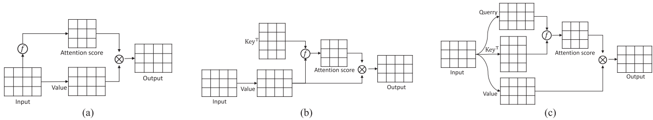
Fig. 2. Illustration of the different attention mechanisms, (a) shows the keyless attention adopted in this work which learns the attention score by operating on the input data itself, (b) is a form of key-value attention in which the attention score is calculated by requiring a Key matrix, (c) illustrates the self-attention introduced in the Transformer model [53] where the attention score is obtained via the key-query relationship and then mapped to the Value matrix. Together, the key-query pair can be regarded as the ‘key’ in the attention mechanism. (a) Keyless. (b) Key-value. (c) Key-query-value.
