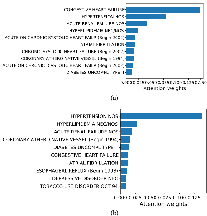
Fig. 6. Diagnosis attention score interpretation by different groups of patients. (a) shows the top ten diagnosis codes for patients that develop organ failures; (b) are the top ten diagnoses for patients without organ failure. (a) Patients with organ failures. (b) Patients without organ failures.
