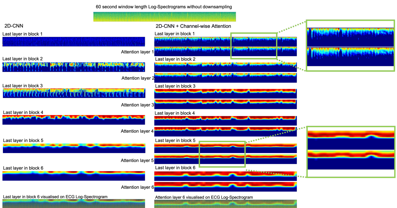
Figure 6. Examples of visual explanations of the features in all different layers of the baseline 2D-CNN method and the proposed 2D-CNN + Channel-wise Attention method. The 60-s window length log-spectrogram of raw ECG data is the input of these two methods. The green rectangle highlights the huge visual difference between the adjacent layers in the proposed method.
