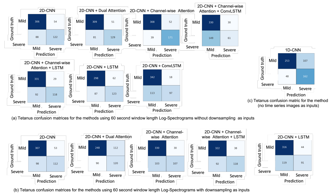
Figure 7. Confusion matrices of the tetanus severity level diagnosis using different deep learning methods: (a) tetanus confusion matrices for the methods using 60 s window length log-spectrograms without downsampling as inputs; (b) tetanus confusion matrices for the methods using 60 s window length log-spectrograms with downsampling as inputs; (c) tetanus confusion matrices for the 1D-CNN method (no time series images as inputs).
