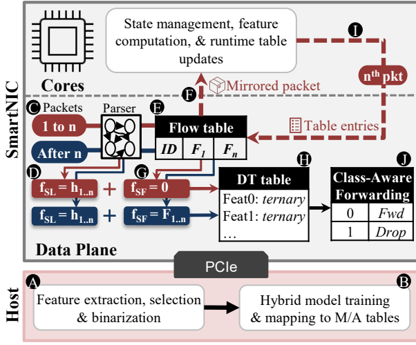
Figure 2: Overview of the H_yNIC system. Steps A to J depict the sequence of events. f_{SL} and f_{SF} respectively denote stateless and stateful feature sets, while h_{1..n} and F_{1..n} are respectively the stateless packet header fields and the stateful features obtained from the flow table.
