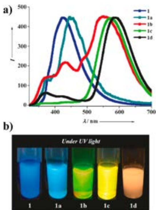
Figure 22. (a) Emission spectra of [\text{Zn}(\text{ndc})(\text{o-phen})]\cdot\text{DMF} (1) MOF before and after the inclusion of aniline (1a), N-methyl aniline (1b), N,N'-dimethyl aniline (1c), and N,N'-dimethyl-p-toluidine (1d), upon excitation at \lambda = 330 nm. (b) Photographs of compounds 1 and 1a–1d after being dispersed in methanol and under UV light irradiation. Reproduced with permission from ref 84. Copyright 2014 John Wiley and Sons.
