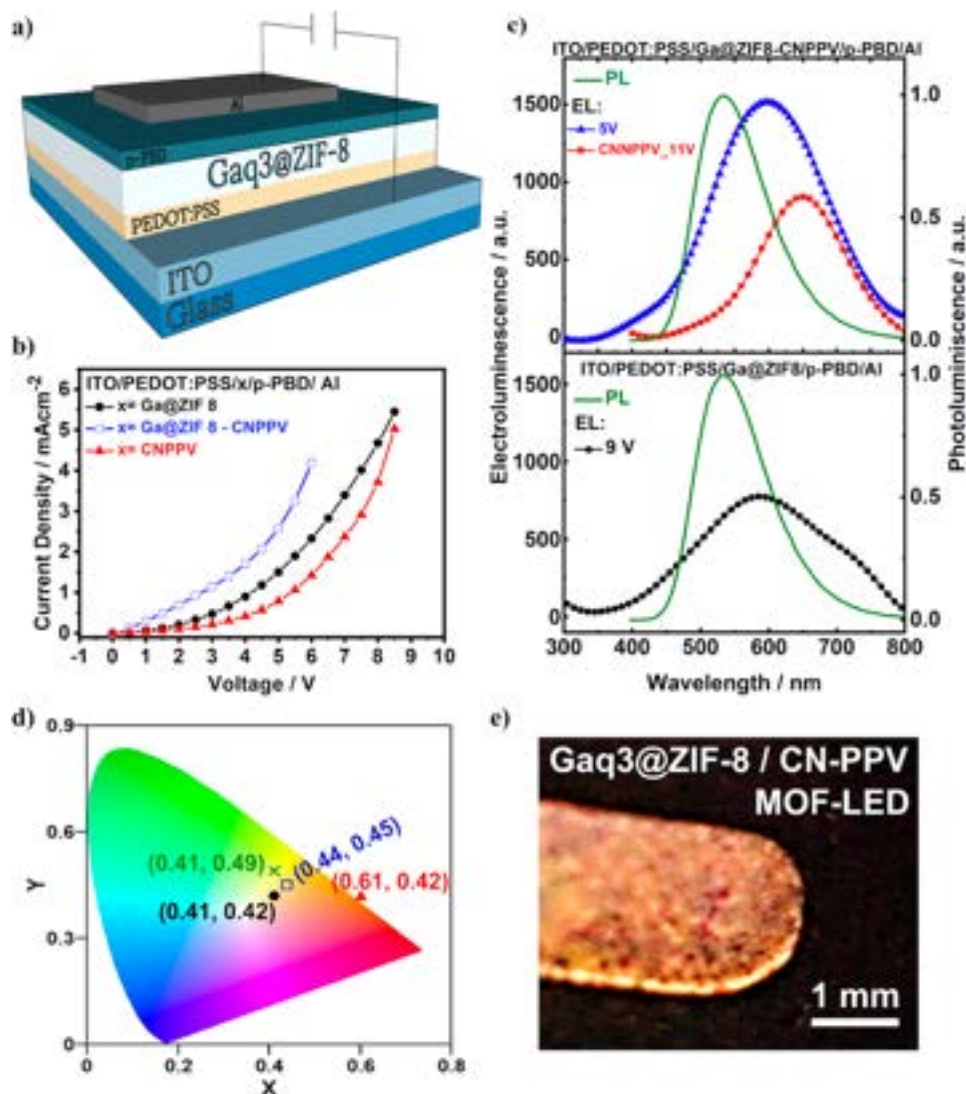
Figure 33. (a) Schematic representation of the multilayer MOF-LED architecture. (b) Current vs voltage curves of the different MOF LEDs and (c) their corresponding electroluminescent spectra. (d) CIE coordinates corresponding to the photoluminescence of \text{GaQ}_3\text{@ZIF-8} (green cross) and the electroluminescence of the different MOF-LEDs ( \text{GaQ}_3\text{@ZIF-8/CNPPV} , blue square; \text{GaQ}_3\text{@ZIF-8} , black dot) and CNPPV-LED (red triangle). (e) Photograph of the MOF-LED device operating at 6 V, in which \text{GaQ}_3\text{@ZIF-8} serves as the electroluminescent layer with the characteristic orange-yellowish emission. Adapted from ref 37. Copyright 2020 John Wiley and Sons.
