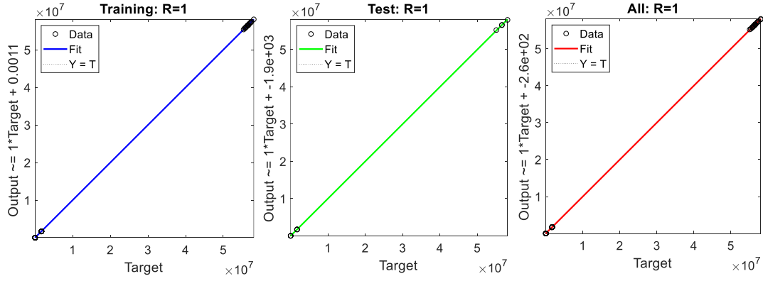
Figure 5 Regression plots
