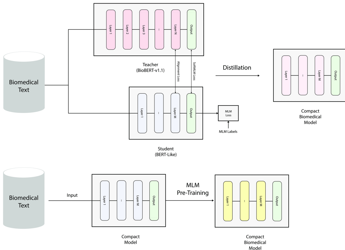
Fig. 1. The two general strategies proposed for training compact biomedical models. The first approach is to directly distil a compact model from a biomedical teacher which in our work is BioBERT-v1.1. The distillation depicted in this figure is the same technique used for obtaining DistilBioBERT. TinyBioBERT and CompactBioBERT, on the other hand, employ different approaches, which are not shown here. The second method involves additionally pre-training a compact model on biomedical corpora. For this approach, we use compact models which have been distilled from powerful teachers, namely, DistilBERT (Sanh et al. , 2019), TinyBERT (Jiao et al. , 2020) and MobileBERT (Sun et al. , 2020)
